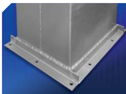
Full weld angle flange connections provide added strength and perfect alignment.
