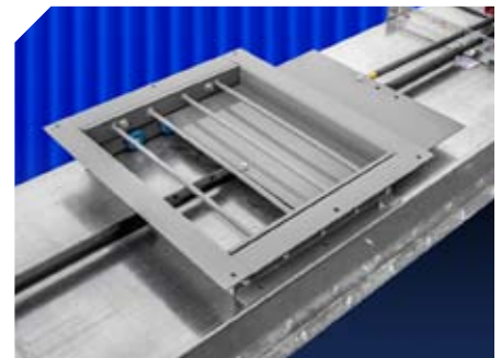
Choice of center and intermediate wells individually positioned for optimal convenience and access. Low profile height on inlets keeps gates positioned to accept the MFS 16" [406 mm] or 18" [457 mm] floor support.
