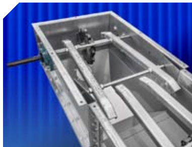
Return rails standard on conveyors with WH124 and WH132 chain. Note: Return rails are not recommended on 8" wide [203 mm] conveyors.
