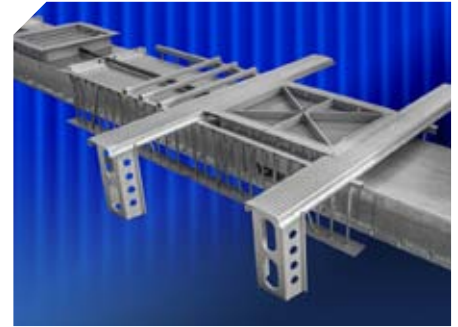
Welded steel supports and center brace span width of conveyor for strong support when used with the MFS floor.
