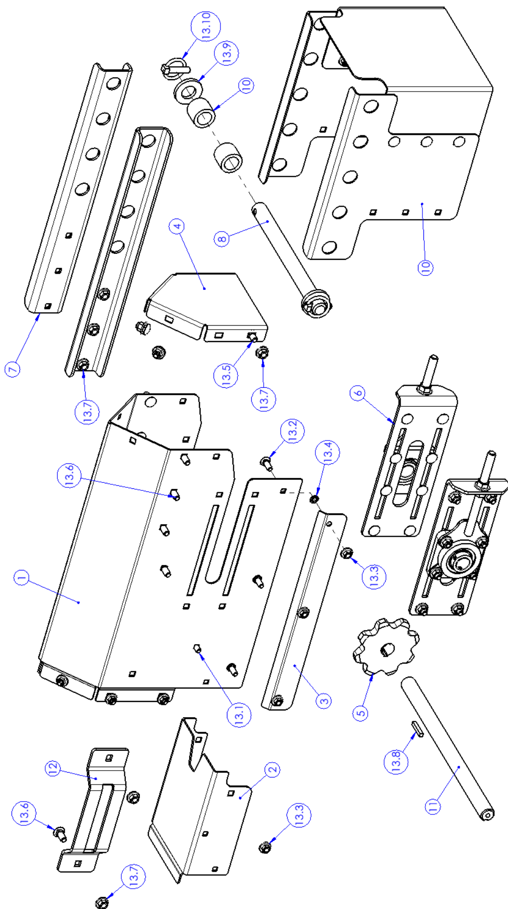
HEAD SECTION ASSEMBLY, ELECTRIC 2K (K714340)
