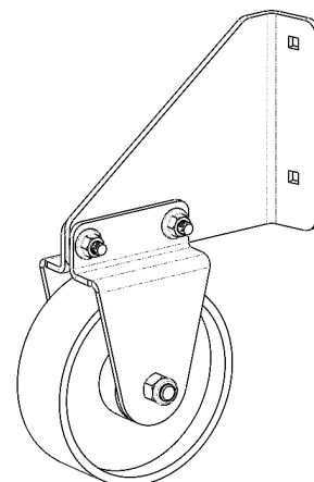
Caster
