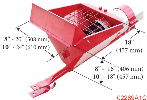
Metal Inlet Hopper
