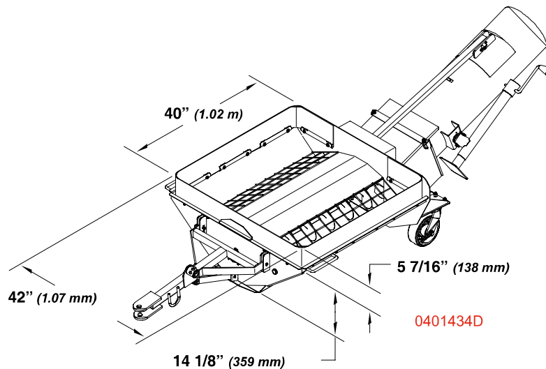
Flexible Bin Hopper
