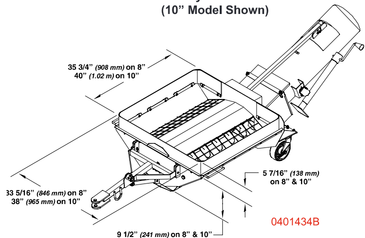
Flexible Bin Hopper
