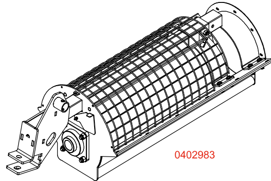
In-Line Style Intake Guard
