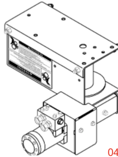
Hydraulic Winch
