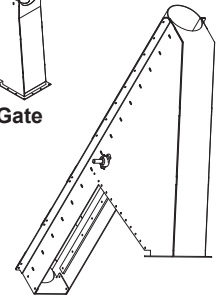
45° Discharge Gate
