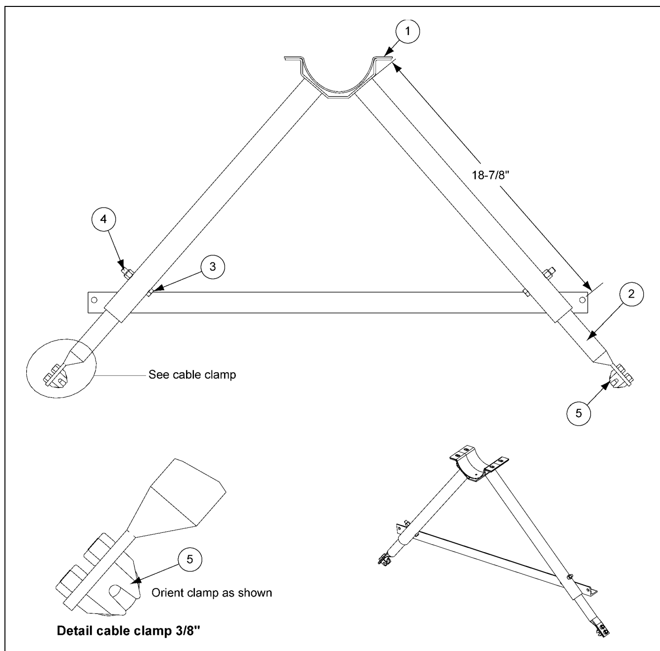
Figure 4 Tube Base Assemblies
